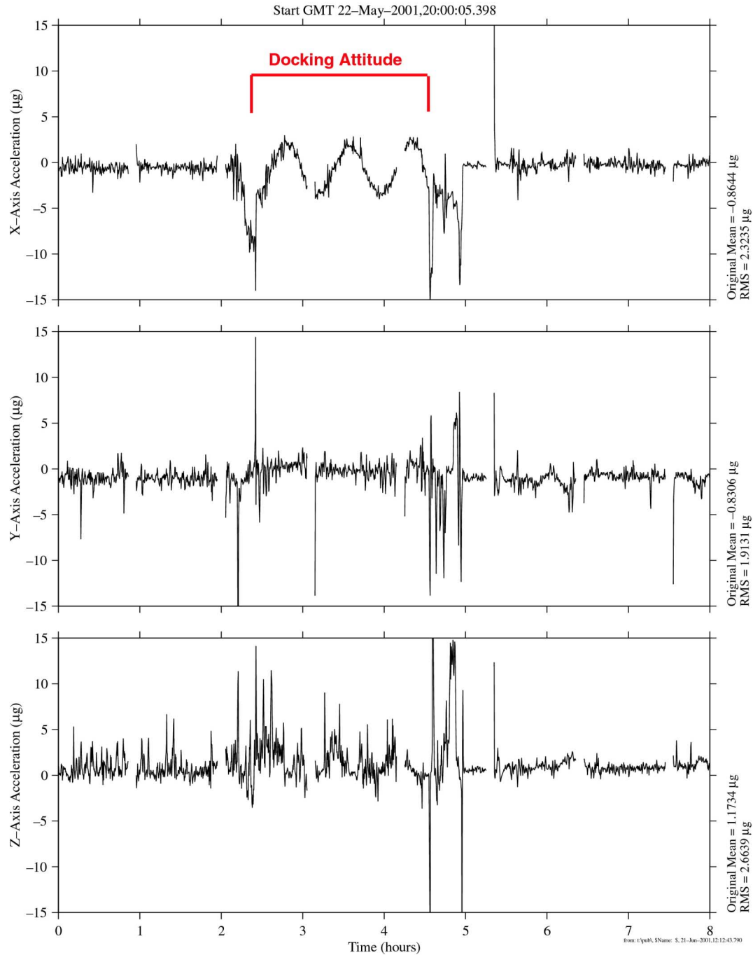
Figure 8.1.3-2 Progress Docking
