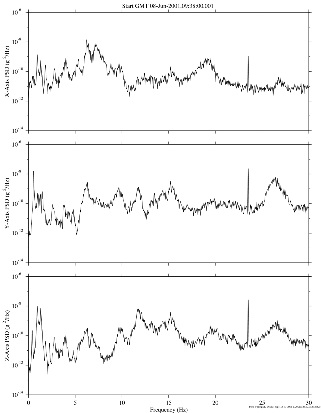
Figure 8.2.1.1-2 PSDs Showing SKV-1 Air Conditioner/Dehumidifier On
