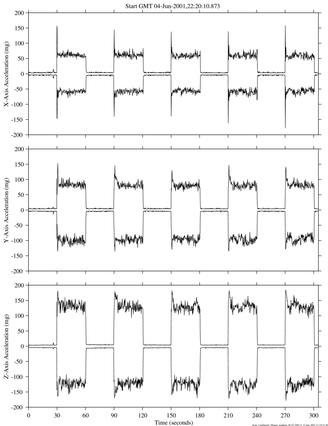
Figure 8.2.2.1-2 Interval Minimum/Maximum of EXPPCS Sample Mix Operation
