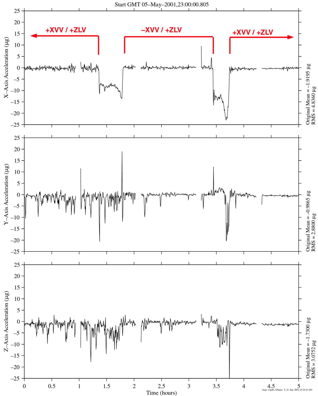
Figure 8.1.3-1 Undocking of Soyuz TM-31
