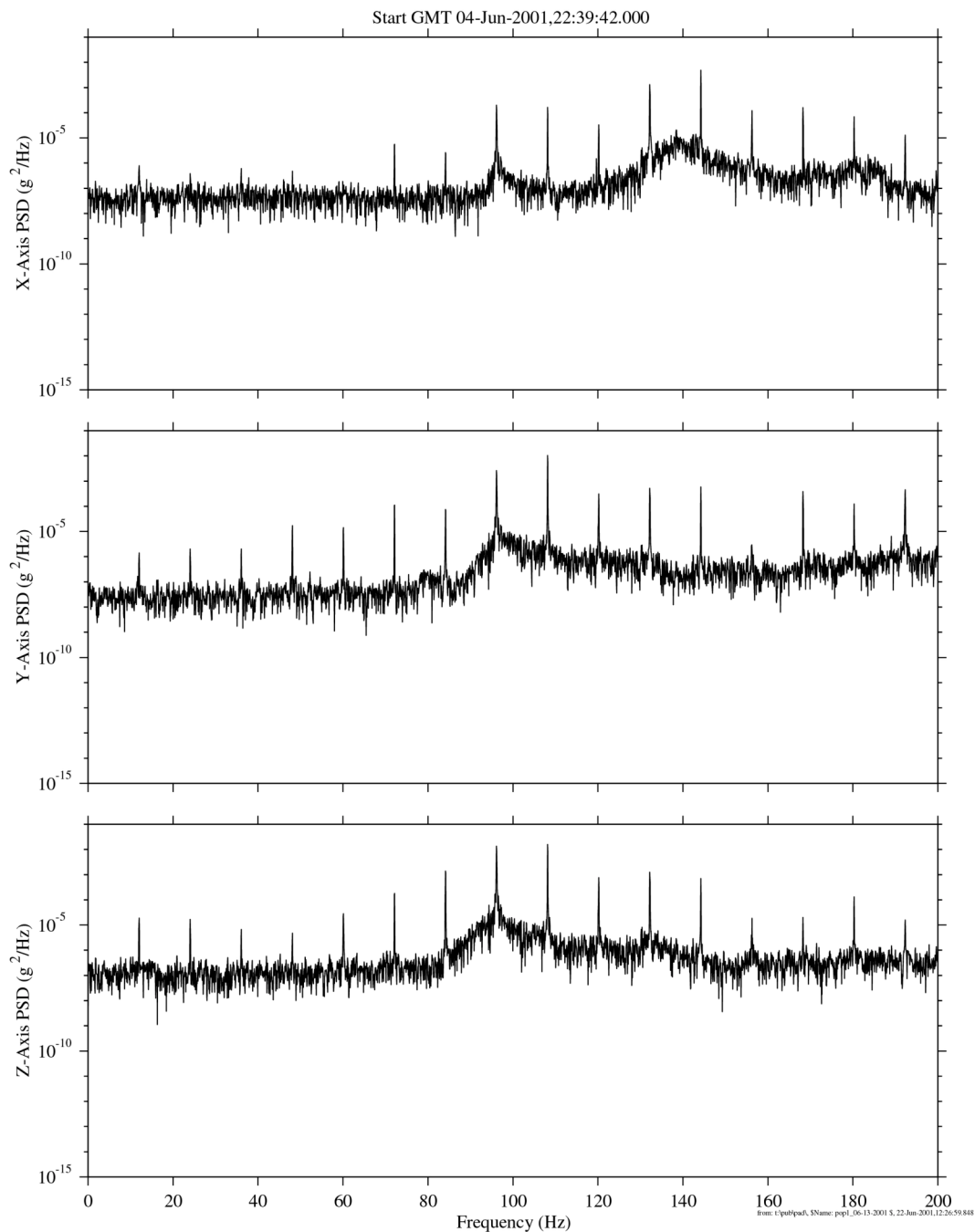
Figure 8.2.2.1-3 PSDs of EXPPCS Sample Mix Operation
