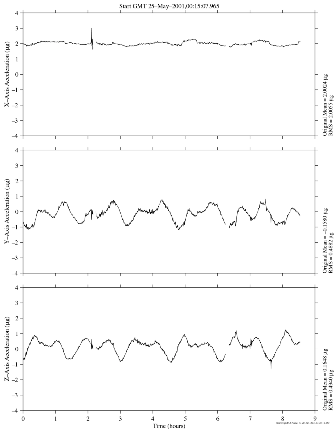
Figure 8.1.2-1 XPOP Attitude
