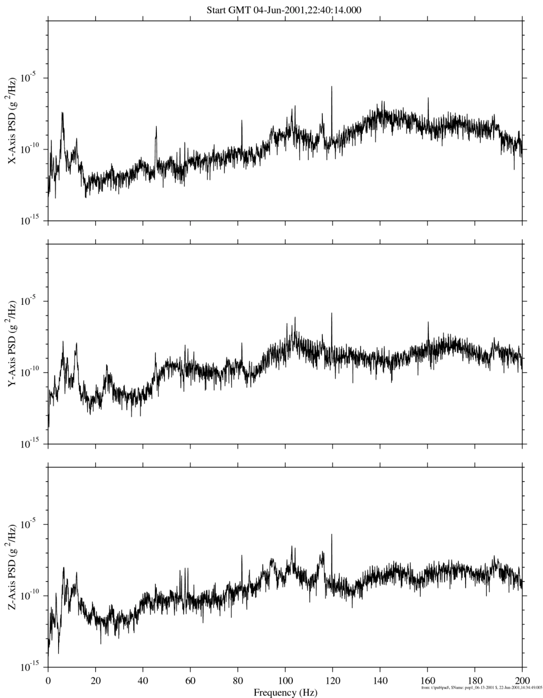
Figure 8.2.2.1-4 PSDs Without EXPPCS Sample Mix Operation
