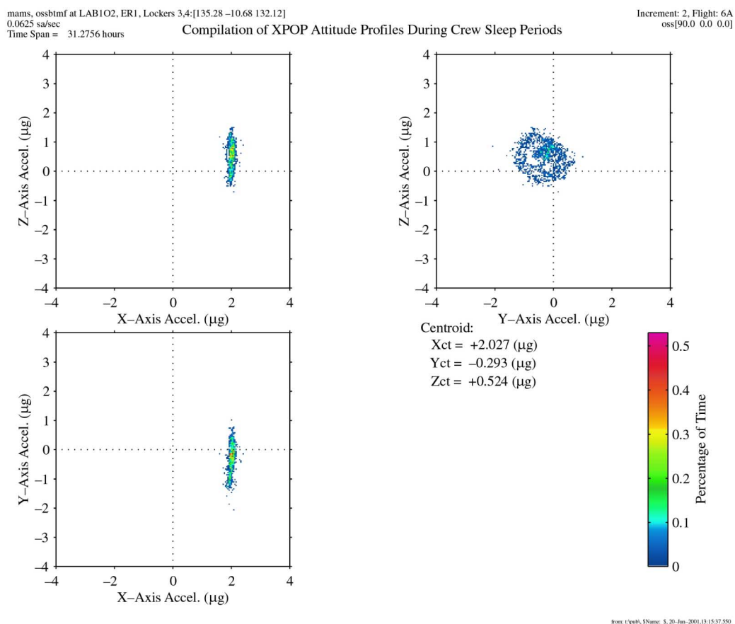
Figure 8.1.2-2 XPOP Attitude Profile for Crew Sleep Periods
