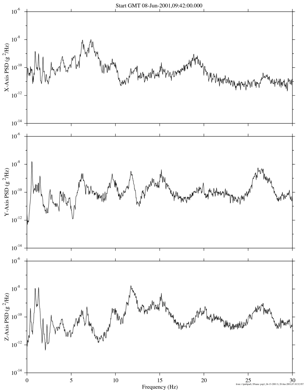
Figure 8.2.1.1-3 PSDs Showing SKV-1 Air Conditioner/Dehumidifier Off
