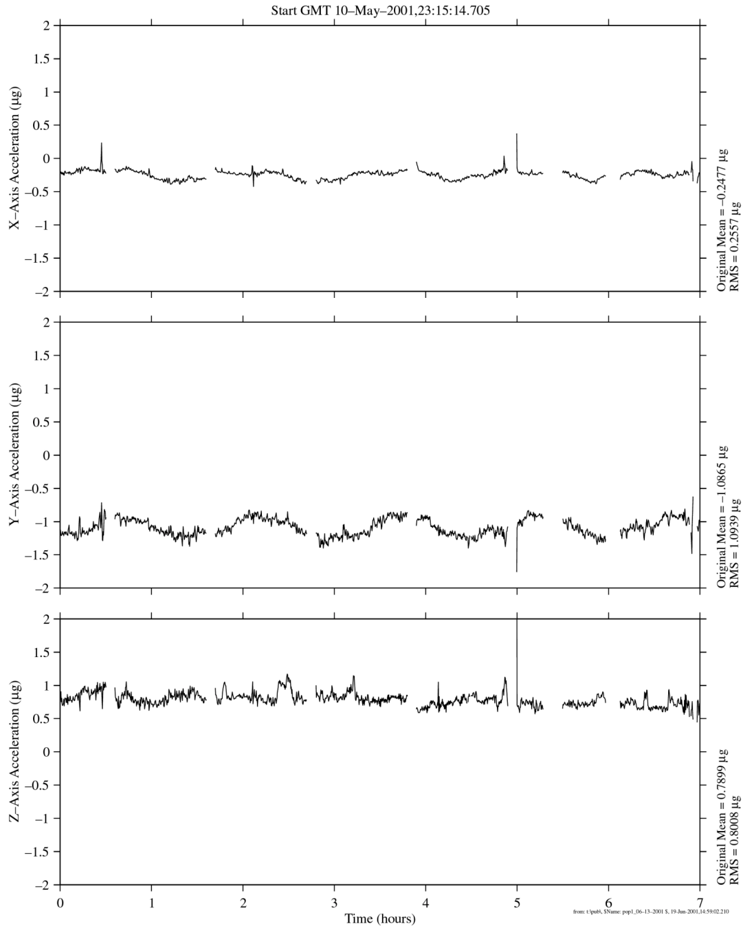
Figure 8.1.1-1 Torque Equilibrium Attitude
